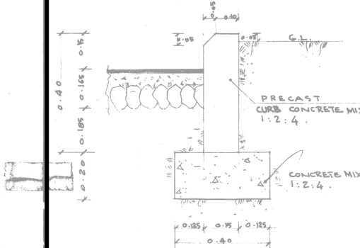
B B PRECAST CURB CONCRETE TYPICAL SECTION
