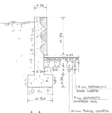
A A RETAINING WALL TYPICAL SECTION
